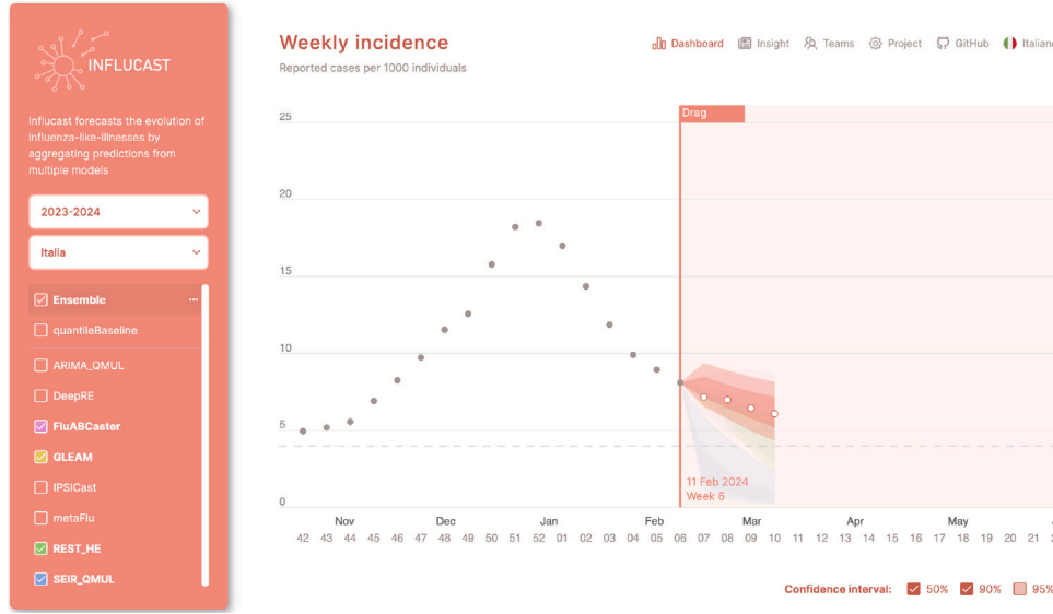
Fig. 5. The Influcast web interface. The visualization dashboard allows displaying the four weeks ahead prediction for the ensemble and for specific models, choosing the season, the location and the prediction intervals to show.
