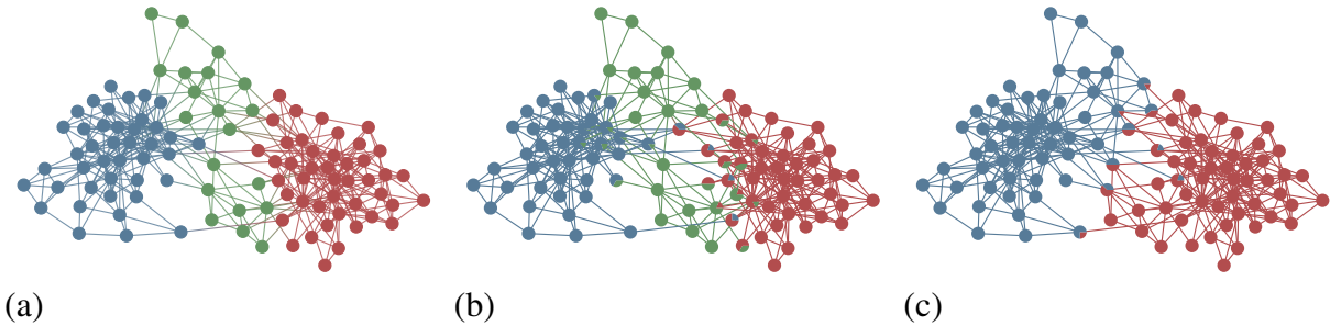
Figure 10. Network of co-purchase of books about US politics [66], with groups inferred using (a) the non-overlapping DC-SBM, with description length \Sigma \approx 1,938 bits, (b) the overlapping SBM with description length \Sigma \approx 1,931 bits and (c) the overlapping SBM forcing only B = 2 groups, with description length \Sigma \approx 1,946 bits.
